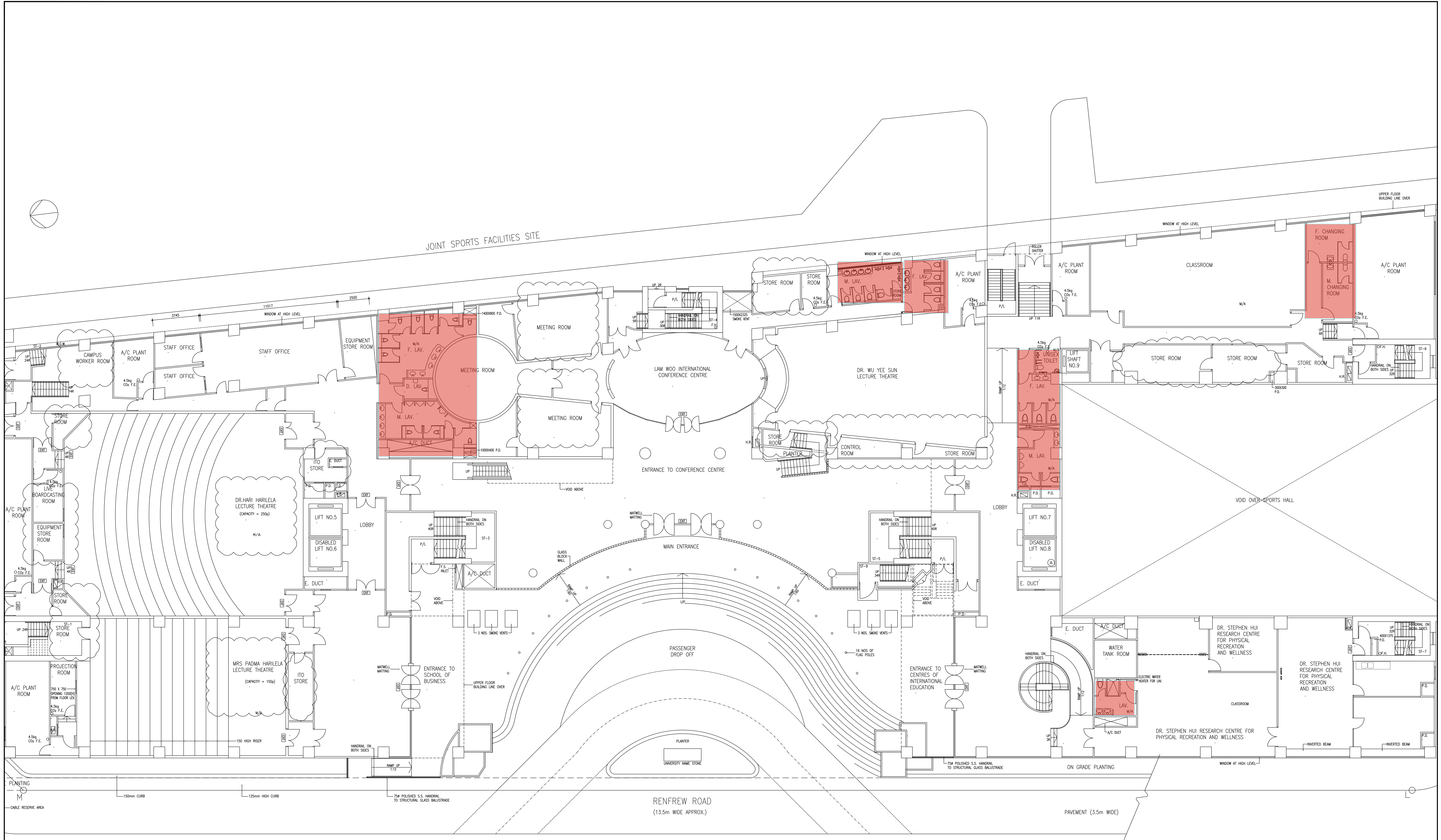
LEVEL 1 PLAN - 34.0 TEACHING ACCOMMODATION/CONFERENCE CENTRE
