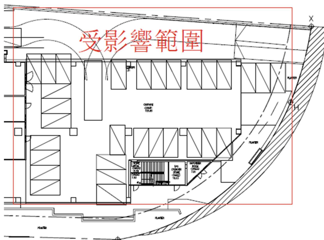
Layout plan of G/F
